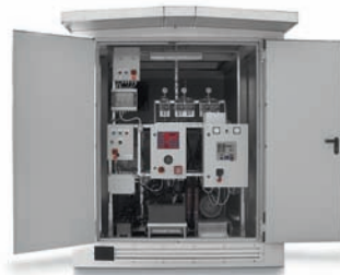
UNI11292 - EN12845 - UNI10779 EXTERNAL PREMISES FOR FIRE FIGHTING UNITS
